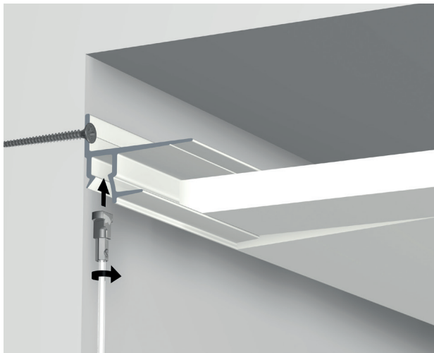
SHADOWLINE MASONRY (IN COMBINATION WITH DRYWALL)
